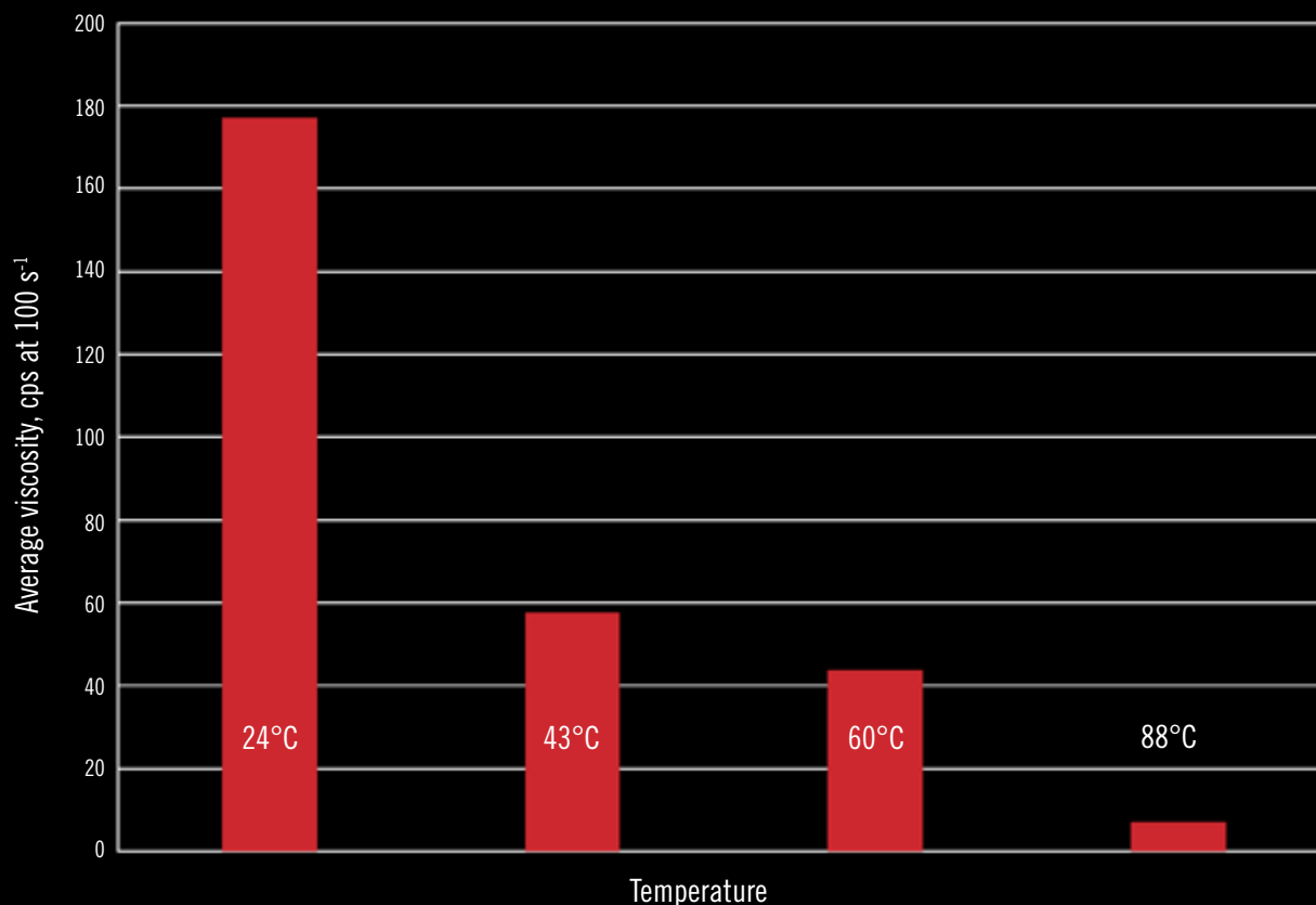
Gel Viscosity of 2 wt% PETROSTEP VES-1 and 1 wt% PETROSTEP VES-C11 in 2 wt% KCl (Grace M5600 Viscometer)
